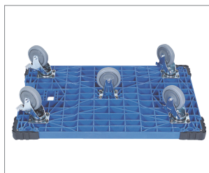
FT-300X-00 (脚轮布置)
